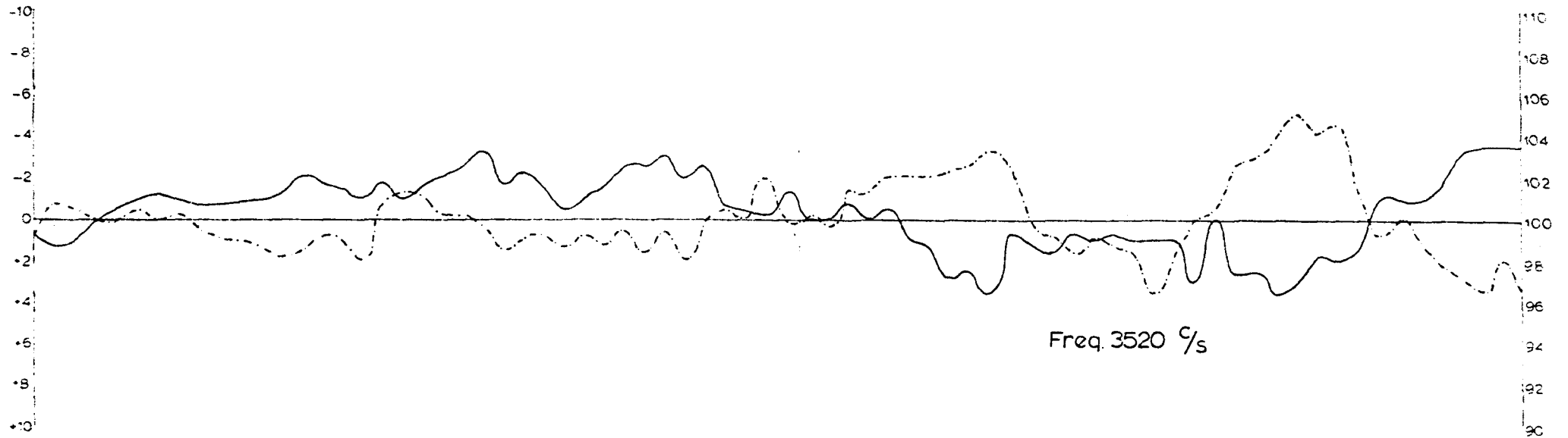
FIG 15 E.M. Traverse 7 Coil Separation 60M. Station Interval 10M. Real Component — Imaginary Component - - -
