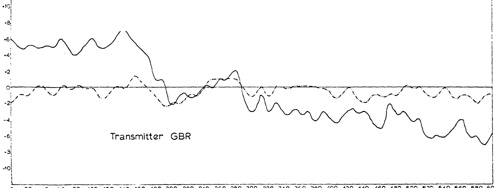
FIG. 19 VLF EM. Traverse 4 Station Interval 10M Real Component — Quadrature Component - - - Direction of Readings →
