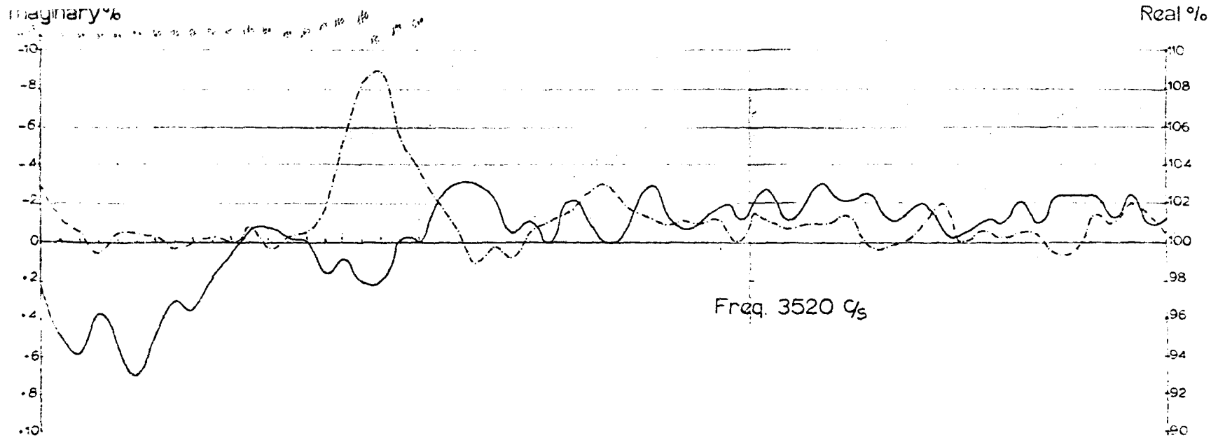
FIG. 12 E.M. Traverse 4 Coil Separation 60M. Station Interval 10M. Real Component — Imaginary Component - - -
