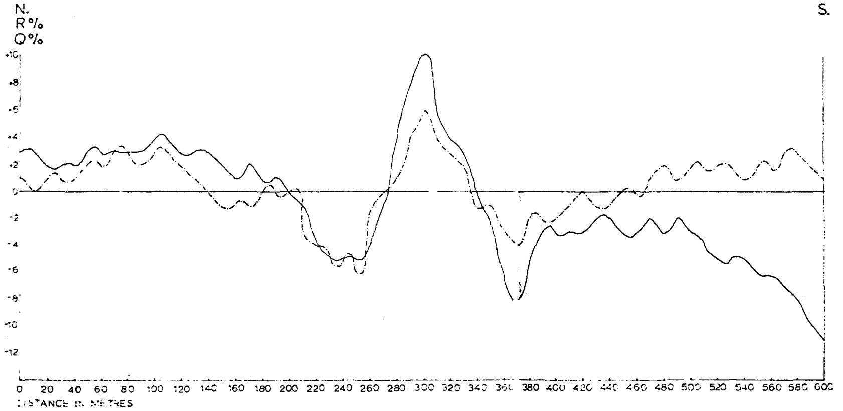
FIG. 7 VLF EM Traverse over Little Eggeshope Vein Transmitter NAA Station Interval 10M. Real Component — Quadrature Component - - - Direction of Readings →
