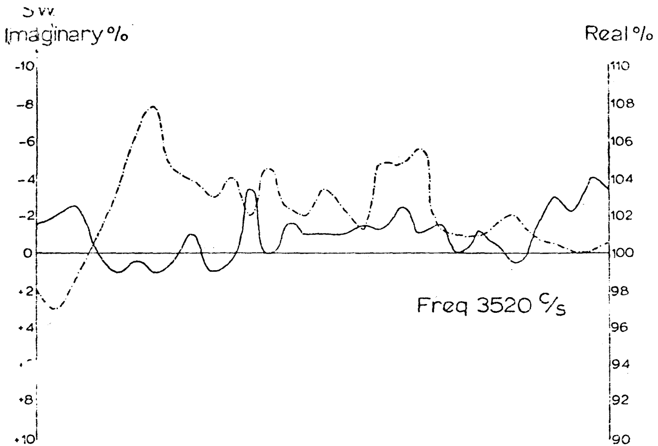
FIG. 11 E.M. Traverse 3 Coil Separation 60M Station Interval 10M Real Component — Imaginary Component - - - -
