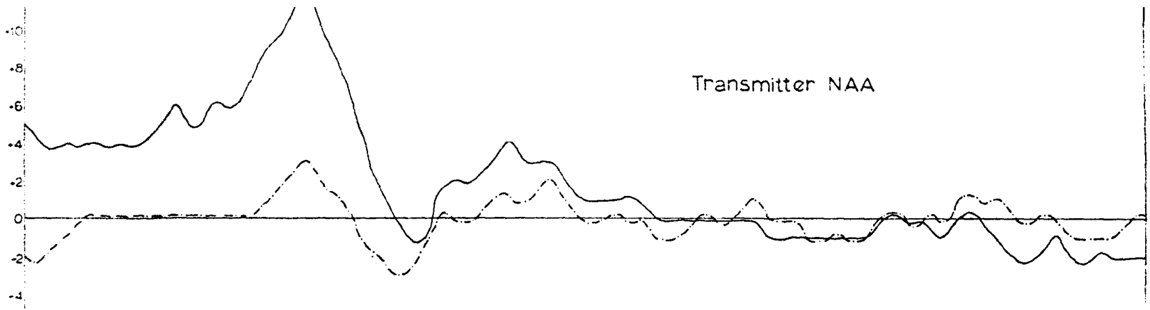
FIG. 19 VLF EM. Traverse 4 Station Interval 10M Real Component — Quadrature Component - - - Direction of Readings →
