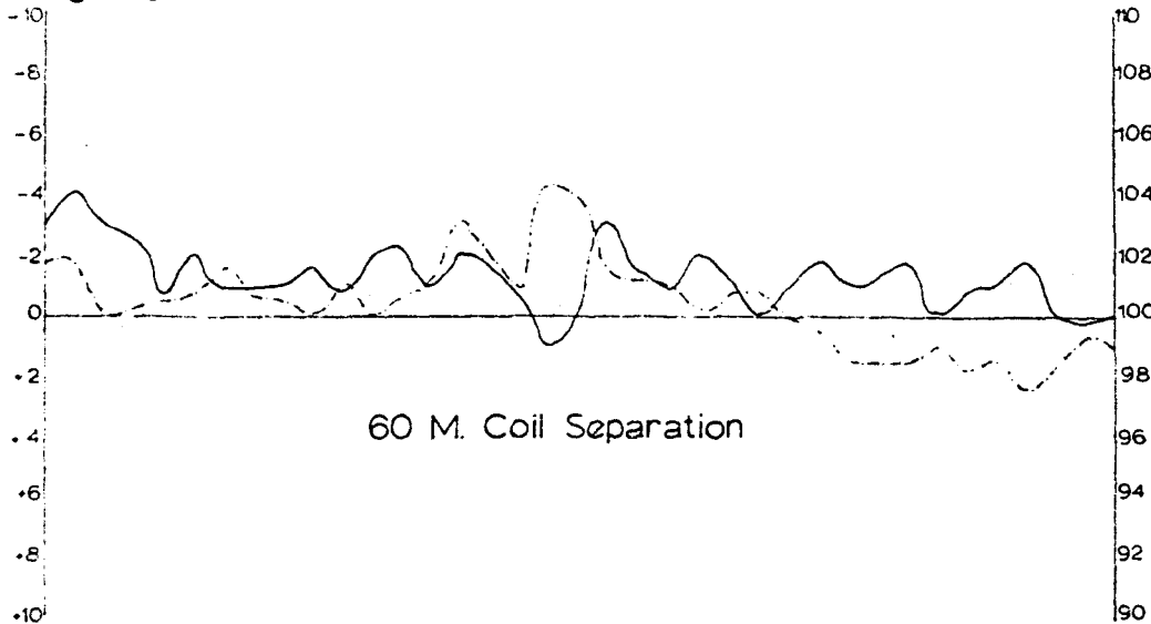
FIG. 14 E.M. Traverse 6 Station Interval 10 M. Frequency 3520 C/s Real Component — Imaginary Component - - -
