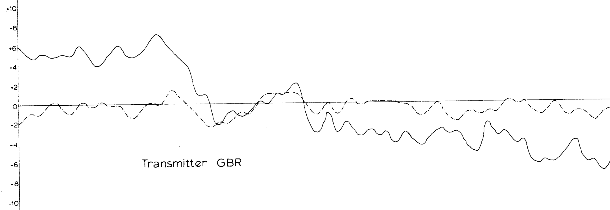
FIG. 19 V.L.F. EM. Traverse 4 Station Interval 10M Real Component — Quadrature Component - - - Direction of Readings →
