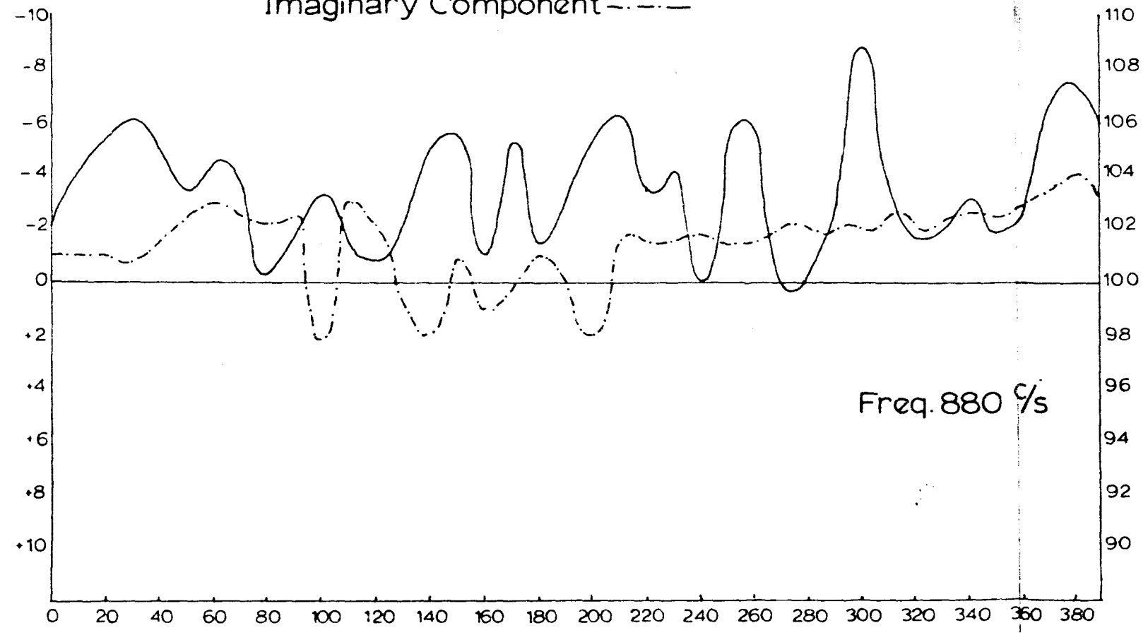
FIG. 16 E.M. Traverse 8 Coil Separation 60M. Station Interval 10M. Real Component — Imaginary Component - - -
