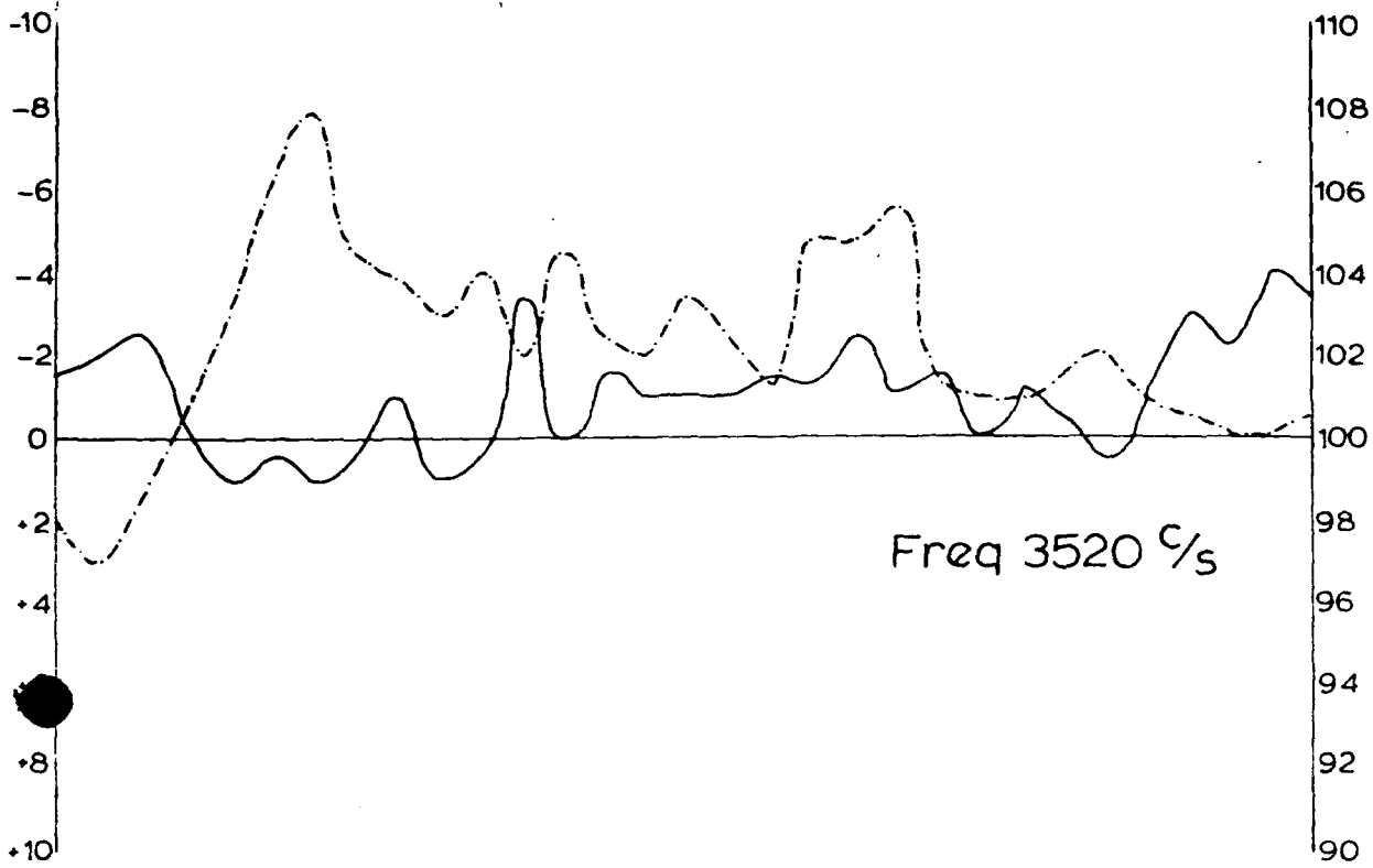
FIG. 11 E.M. Traverse 3 Coil Separation 60M Station Interval 10M Real Component — Imaginary Component - - - -
