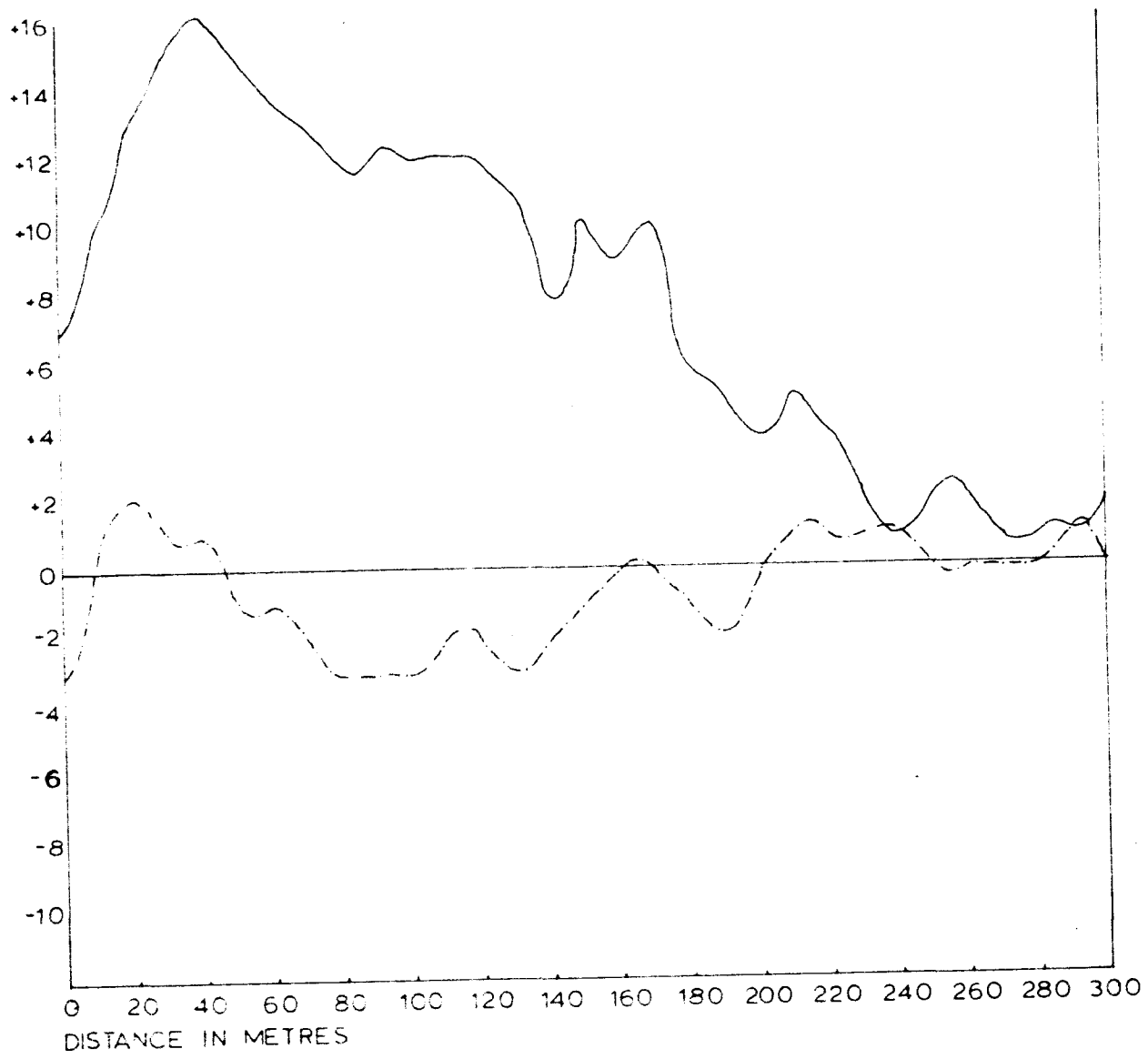
FIG. 18 V.L.F. EM. Traverse 3 Transmitter NAA Station Interval 10M Real Component — Quadrature Component - - - Direction of Readings →
