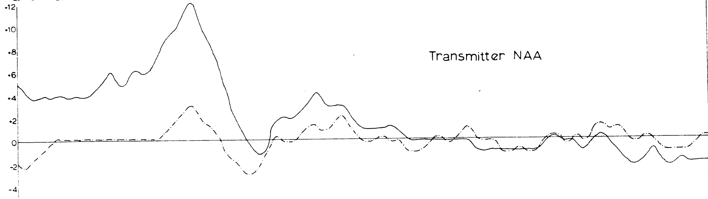
FIG. 19 V.L.F. EM. Traverse 4 Station Interval 10M Real Component — Quadrature Component - - - Direction of Readings →
