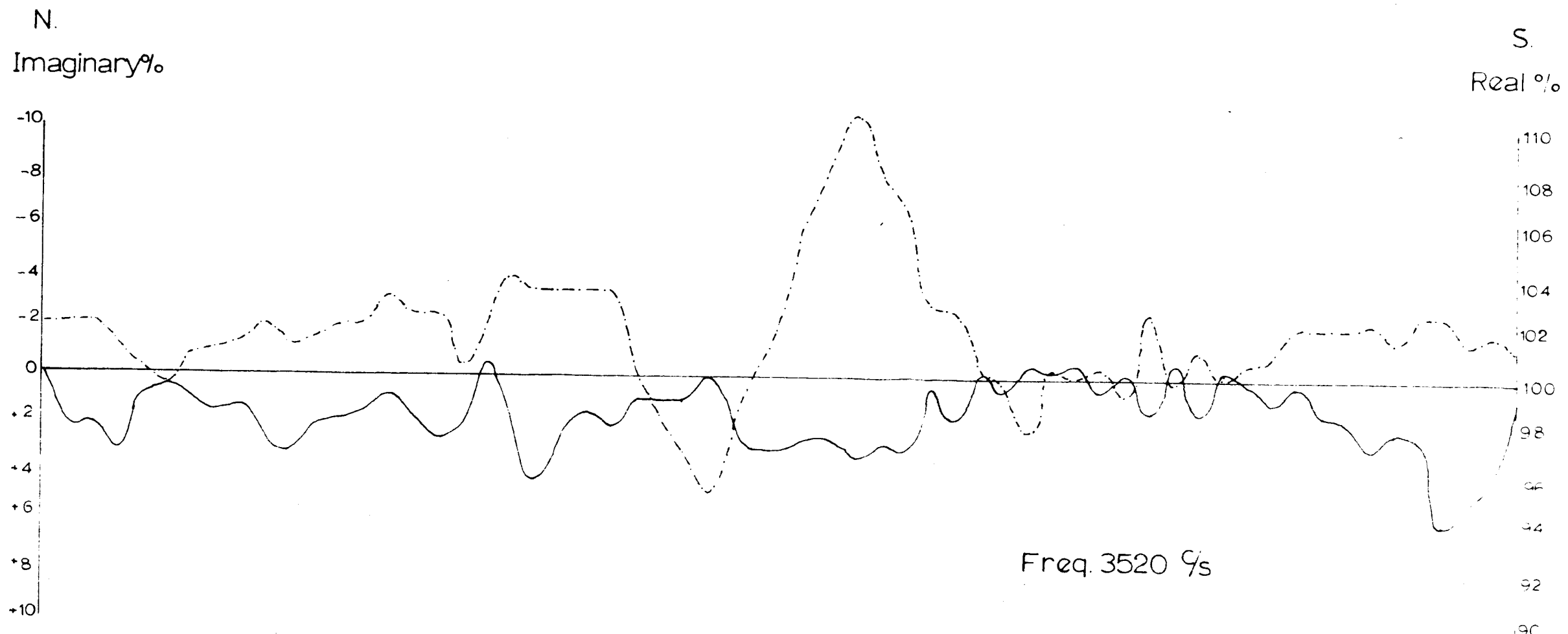
FIG. 4 E.M. Traverse over:- The Little Egglehope Vein.
