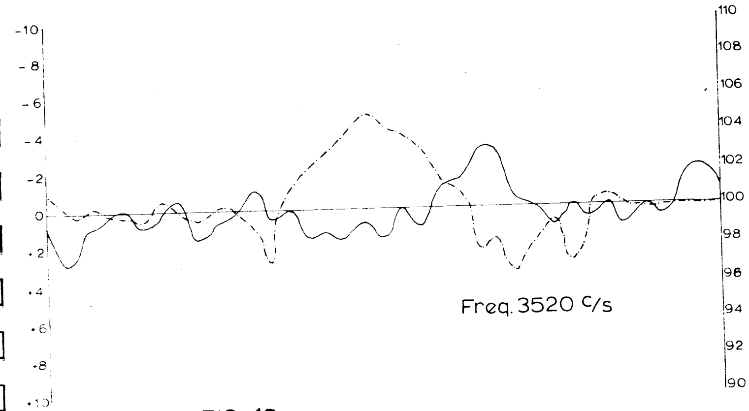
FIG. 13 E.M. Traverse 5 Coil Separation 60M. Station Interval 10M. Real Component. — Imaginary Component. - - -
