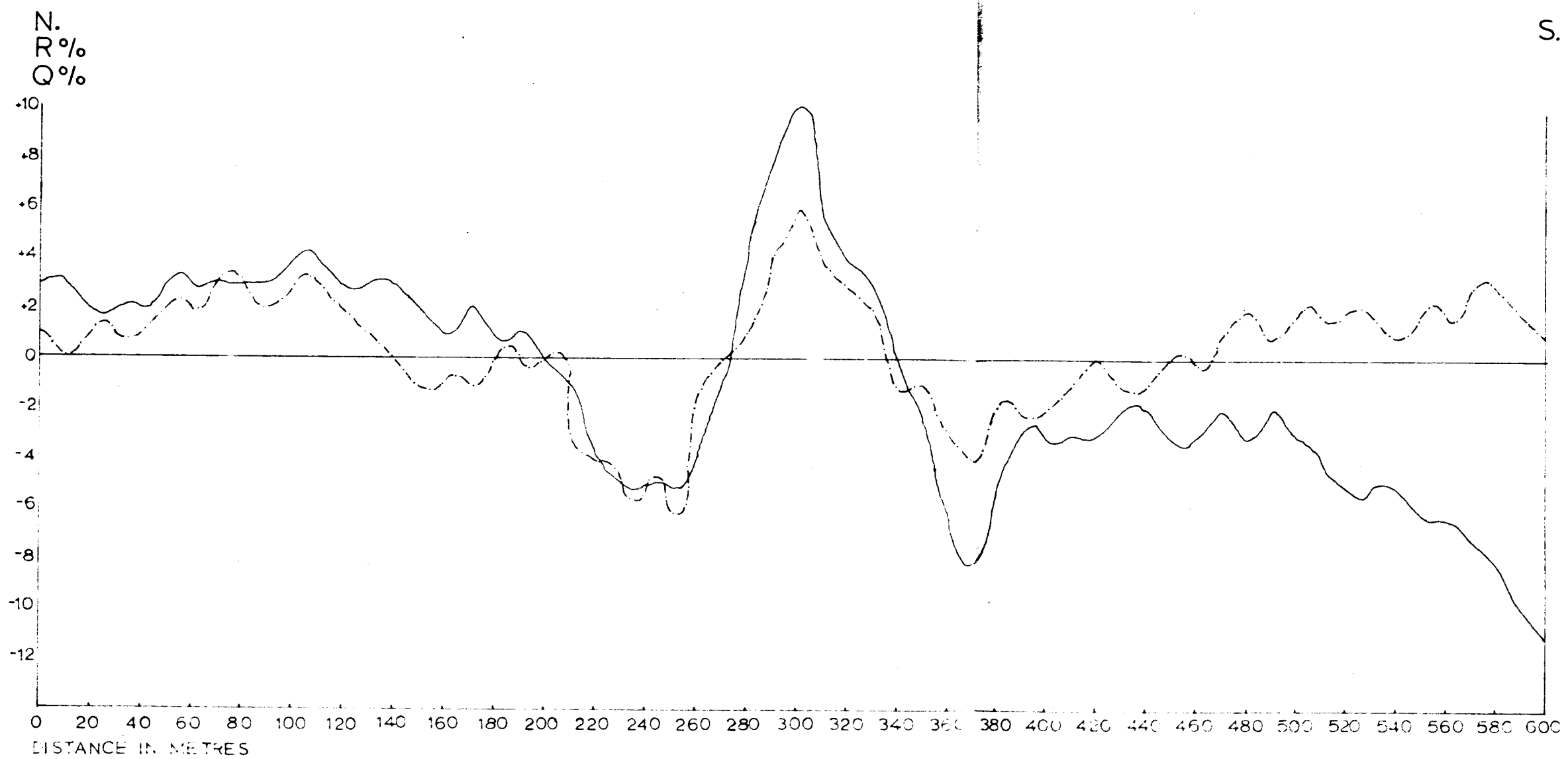
FIG. 7 VLF EM Traverse over Little Egleshope Vein Transmitter NAA Station Interval 10M. Real Component — Quadrature Component --- Direction of Readings →
