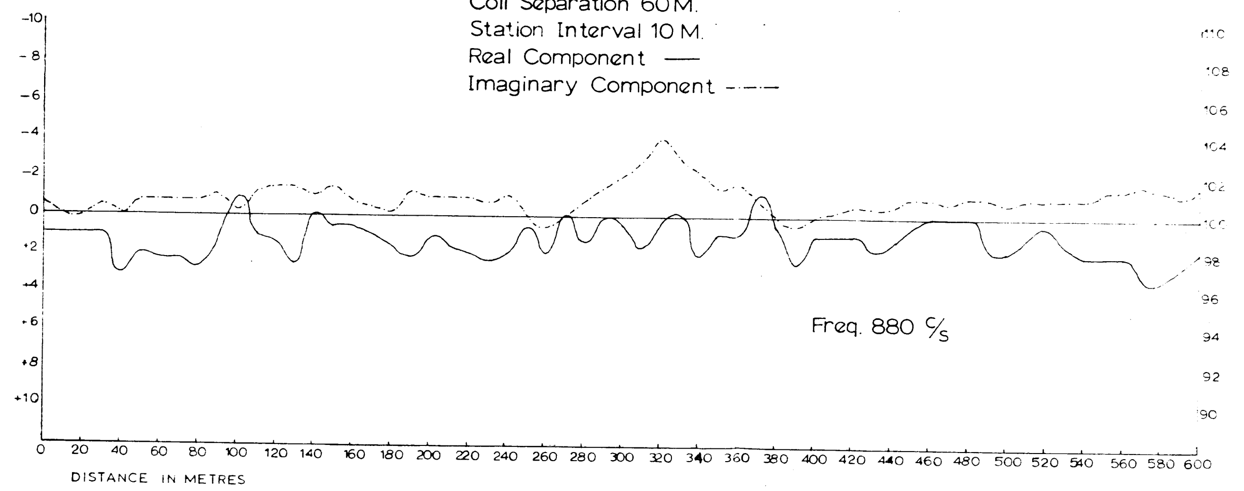
FIG. 4 E.M. Traverse over:- The Little Egglehope Vein.
