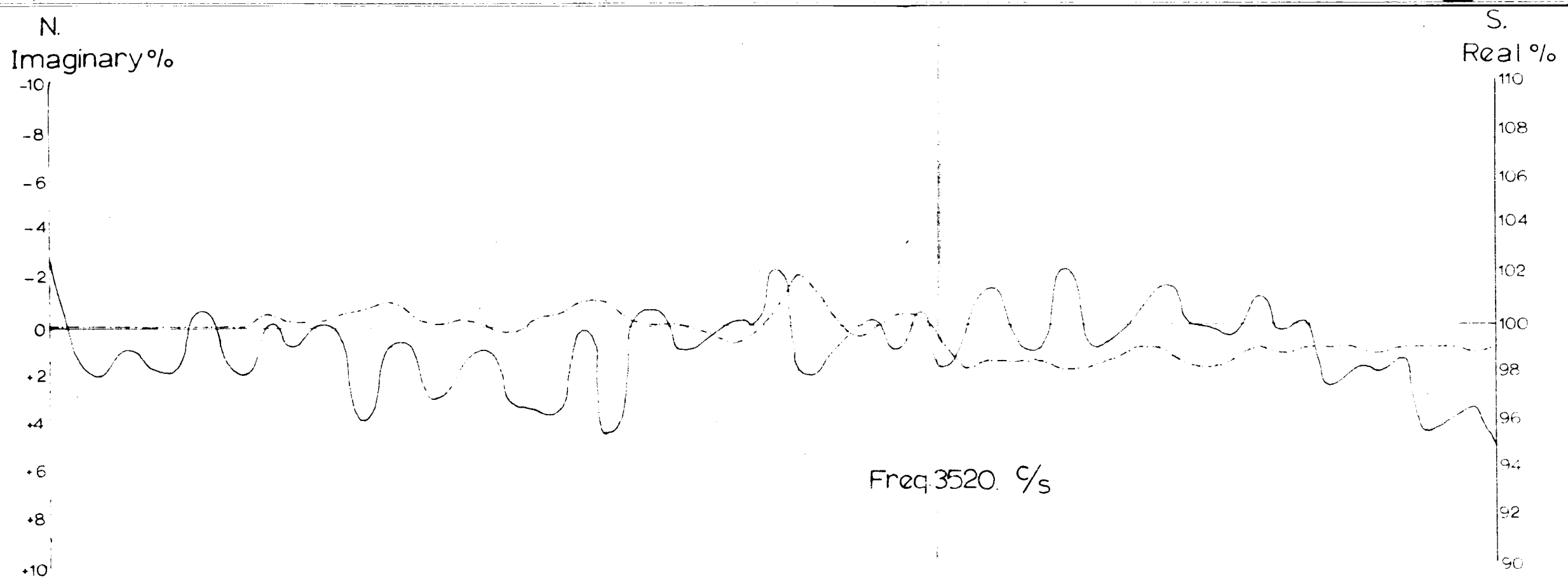
FIG. 5 E.M. Traverse over The Little Egglehope Vein Coil Separation 30 M. Station Interval 10 M. Real Component — Imaginary Component - - -
