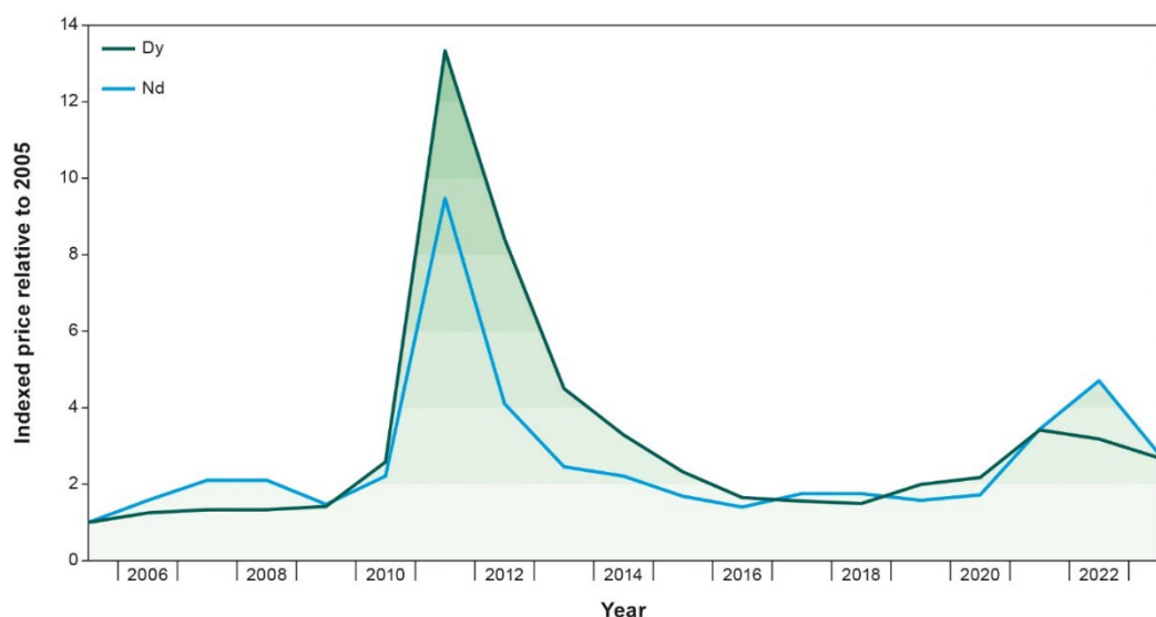
Figure 13 Average annual prices for Dy and Nd indexed to 2005. Data from USGS (U.S. Geological Survey, 2024b; U.S. Geological Survey, 2024a). Note: average annual prices do not show price changes at monthly or shorter time scales. BGS © UKRI.
